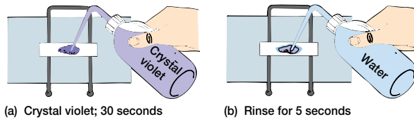
Figure 8.3 Gram-stain Procedure.
