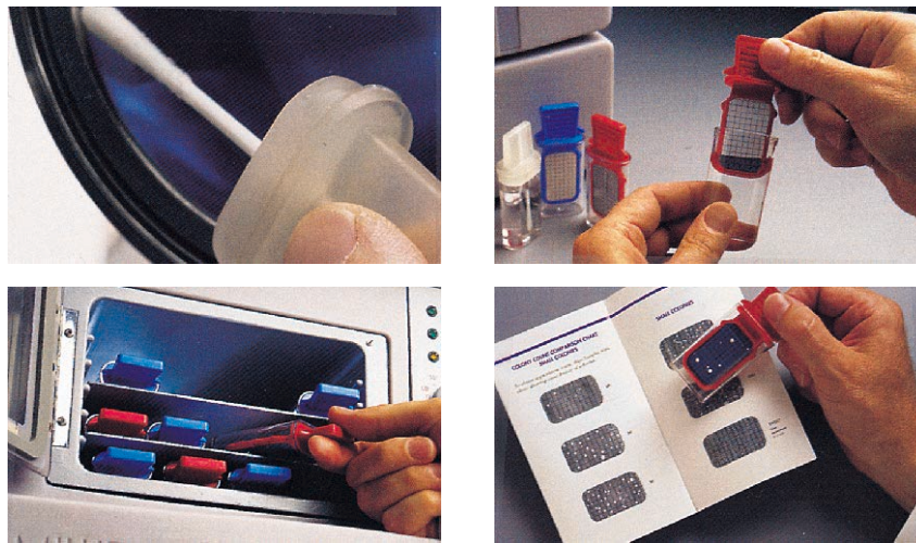
Figure 44.2 The Self-Contained Membrane Filter Test (Millipore). (a) To sample surfaces, wipe the surface with the swab; return the swab to the plastic case containing sterile buffer; shake 30 times; discard the swab. (b) To sample liquids, fill the case with the fluid to be tested; insert the sampler into the case and lay it horizontally with the membrane side down for 30 seconds; pour out the test fluid. (c) Reinsert the sampler into the case and incubate with the membrane-side down. (d) Count the colonies or make a quick comparison using the comparison chart provided in the package figure 44.3.
